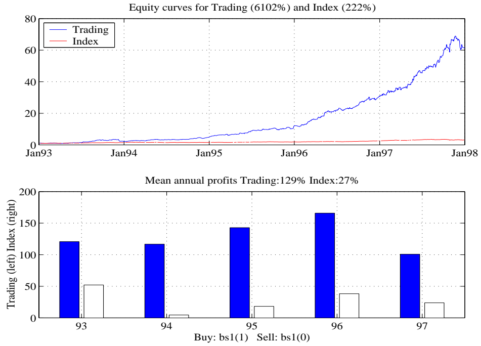
Fig. 4. Performance for the simulated trading with stock picking based on 1-day rank predictions as shown in Figure 3. The top diagram shows the equity curves while the lower diagram displays the annual profits. The trading outperforms the benchmark index consistently every year.
