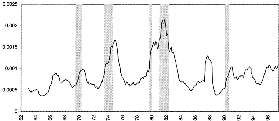
Figure 3. Annualized industry-level volatility IND. The top panel shows the annualized variance within each month of daily industry returns relative to the market, calculated using equations (18) and (19), for the period from July 1962 to December 1997. The bottom panel shows a backwards 12-month moving average of IND. NBER-dated recessions are shaded in gray to illustrate cyclical movements in volatility.
