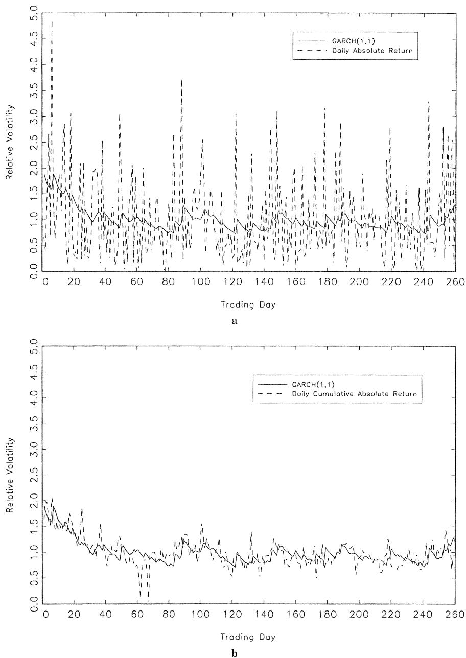
Figure 2. Daily GARCH(1,1) volatility forecasts versus ex post return variability measures. The figures plot the conditional return standard deviation forecasts from an MA(1)-GARCH(1,1) model for the daily deutsche mark-dollar returns from October 1, 1992 through September 29, 1993, along with the corresponding realized absolute daily returns (Figure 2a) and the corresponding cumulative absolute five-minute returns (Figure 2b). All series have been normalized to average unity over the one-year sample.
