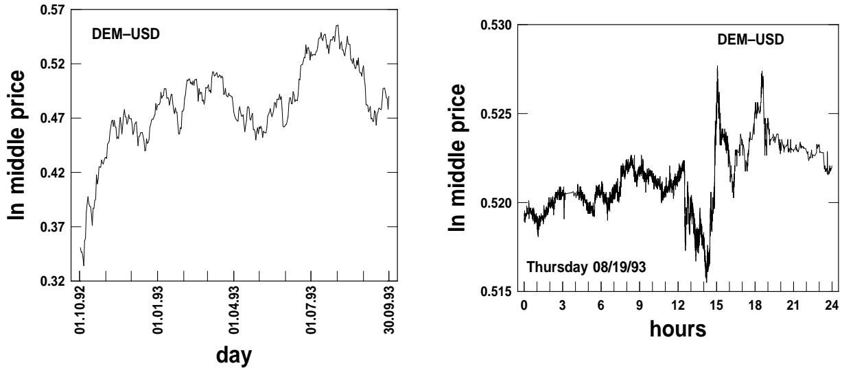
Figure 2: left) The daily logarithmic middle price record for DEM-USD. The prices plotted are those quoted closed to 3 P.M. Greenwich Mean Time. The right) plot is the intra-day logarithmic middle price record on Thursday August 19, 1993. Note the anti-correlations on the small time scales in the plot on the right. The empirical Hurst exponent is H = 0.45 on these short time scales.
