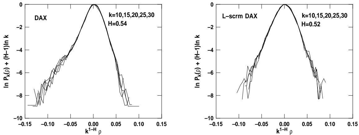
Figure 4: Left ) The basic distribution Q for the DAX stocks in the period November 3, 1986 till August 4, 1993. The rescaling rule Equation 3 is used with the self-similarity exponent H = 0.54 . Right ) The same analysis, however, with DAX stocks in which the daily returns have been scrambled to get rid of correlations. The change in shape shows that correlations between the daily returns do play a role in the price formation. The tails are a bit shorter, because a shorter period has been used – November 3, 1986 till September 7, 1992.
